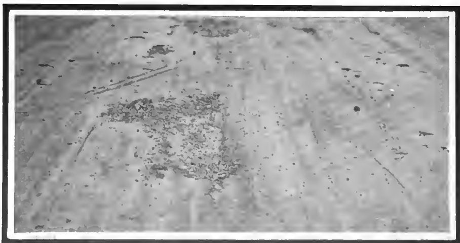
Where a calk wound has allowed water to penetrate, causing destruction of the road surface
